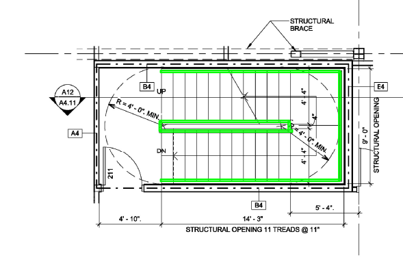
C6 LEVEL 02 - WEST STAIR 1/4" = 1'-0"
