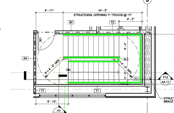
E3 LEVEL 03 - EAST STAIR 1/4" = 1'-0"
