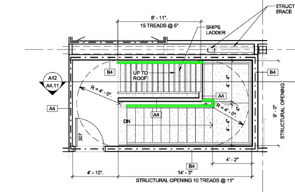
E6 LEVEL 02 - WEST STAIR 1/4" = 1'-0"
