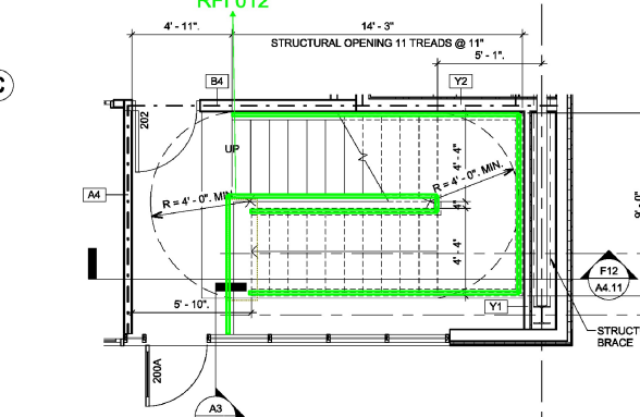
C3 LEVEL 02 - EAST STAIR 1/4" = 1'-0"
