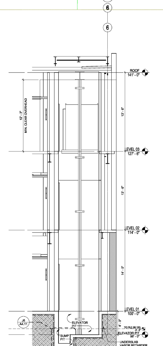
A9 ELEVATOR SECTION 1/4" = 1'-0"
