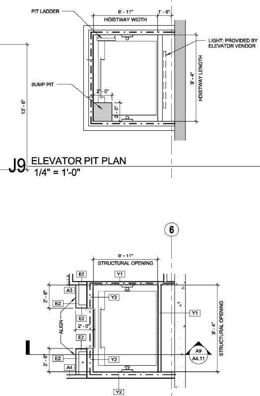
J9 ELEVATOR PIT PLAN 1/4" = 1'-0"
