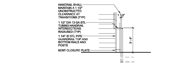
G3 STAIR RAILING AT TRANSITION 3/8" = 1'-0"
