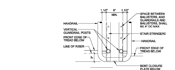
G6 HANDRAIL AND GUARDRAIL AT LANDING PLAN 1 1/2" = 1'-0"
