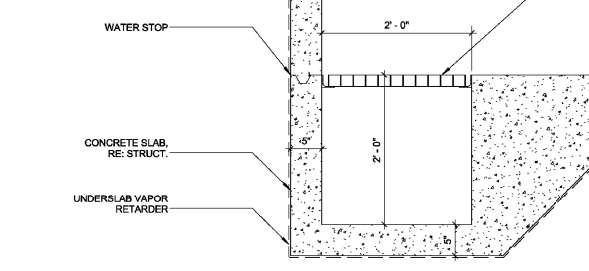
J6 ELEVATOR SUMP DETAIL 1" = 1'-0"
