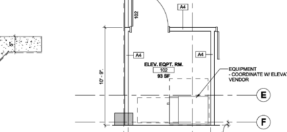
J3 ELEVATOR EQUIPMENT ROOM 1/4" = 1'-0"
