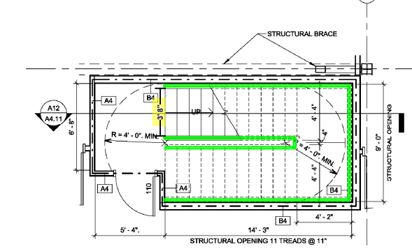
A6 LEVEL 01 - WEST STAIR 1/4" = 1'-0"
