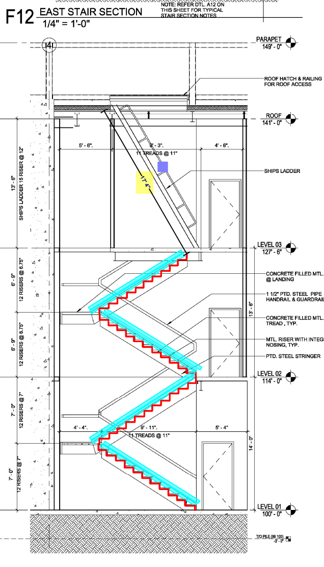
A12 WEST STAIR SECTION 1/4" = 1'-0"
